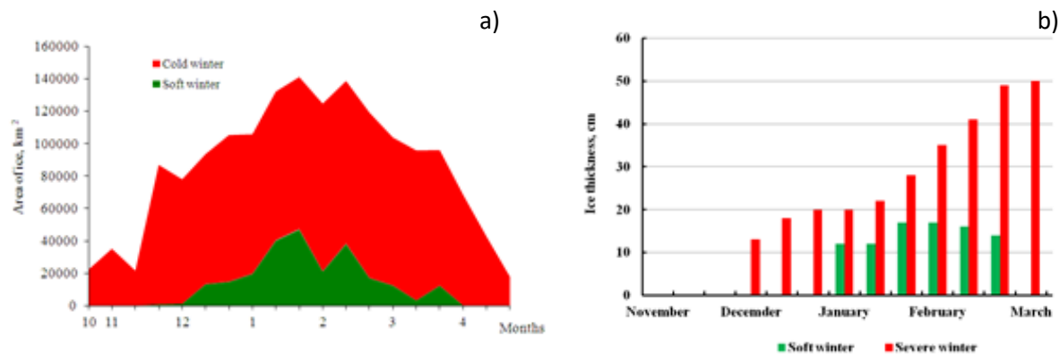
Figure 5. Ice conditions in mild and severe winters: a) area of ice at various winters and b) ice thickness in mild and severe winters
