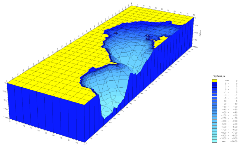
Figure 3. Bathymetry and the longitudinal cross-section of the Caspian Sea
