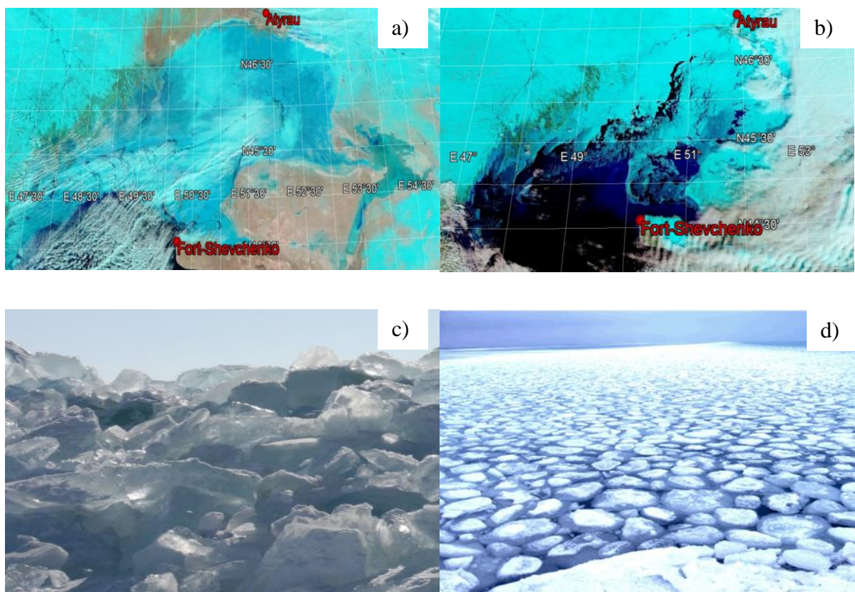
Figure 4. Ice conditions on the Caspian Sea a) cold winter 24th of January 2012 and b) Ice soft winter 30th of January 2016 (Image from the MODIS Rapid Response Project at NAGA/GSFC); show ice large ridges and hummocks (up to 10 m in height) c) and ice on the Northern Caspian Sea d)
