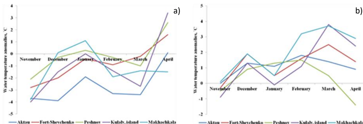
Figure 10. Time series of water temperature anomalies during a) the severe winter 2011-2012 and b) the mild winter 2015-2016
