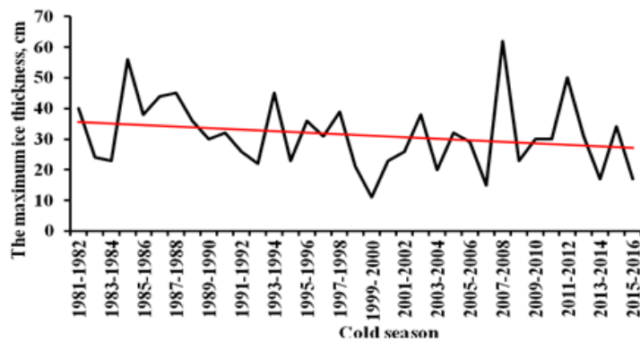
Figure 8. Maximum of ice thickness at the Peshnoy Station for the period 1981-2016
