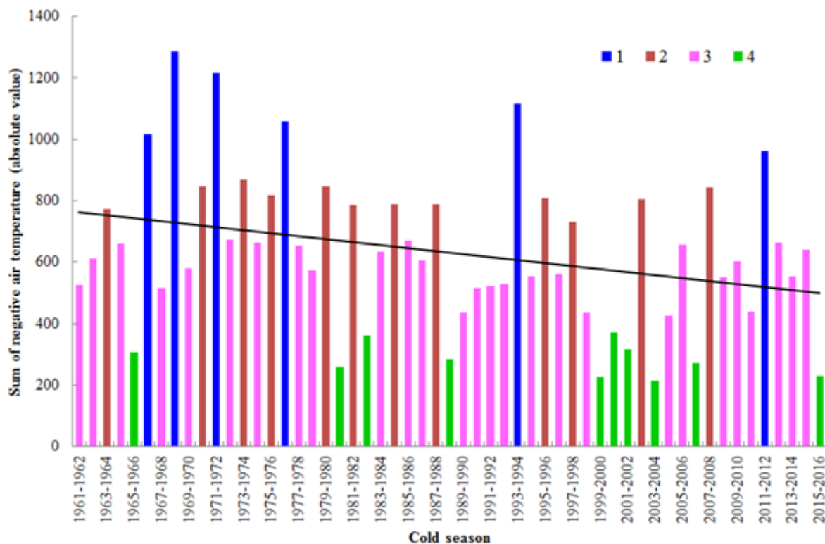
Figure 7. Sums of negative temperatures in the winter season (1961 - 2016), according to the Peshnoy Station. 1 - Very severe, 2 - Severe, 3 - Moderate, 4 - Mild
