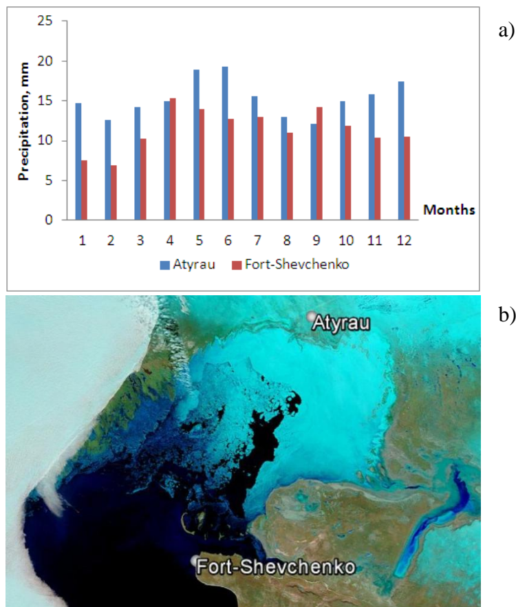
Figure 2. Monthly precipitation (a) at the Atyrau and Fort-Shevchenko meteorological stations (b)
