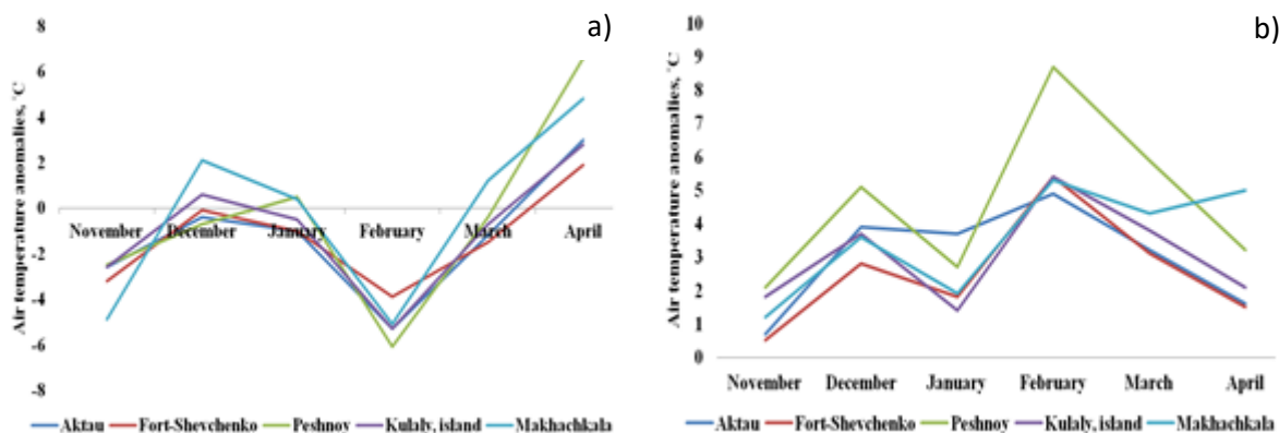
Figure 9 Time series of air temperature anomalies in a), the severe winter of 2011-2012 years and b) in the mild winter of 2015-2016
