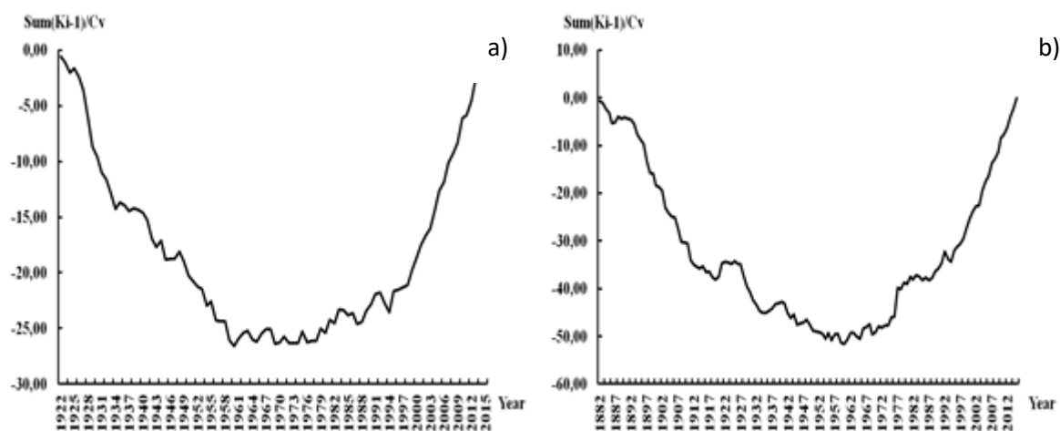
Figure 6. Difference-integral curve of mean annual air temperature at a) Atyrau Station for the years 1922-2015, and b) Fort-Shevchenko Station for the year 1882-2015
